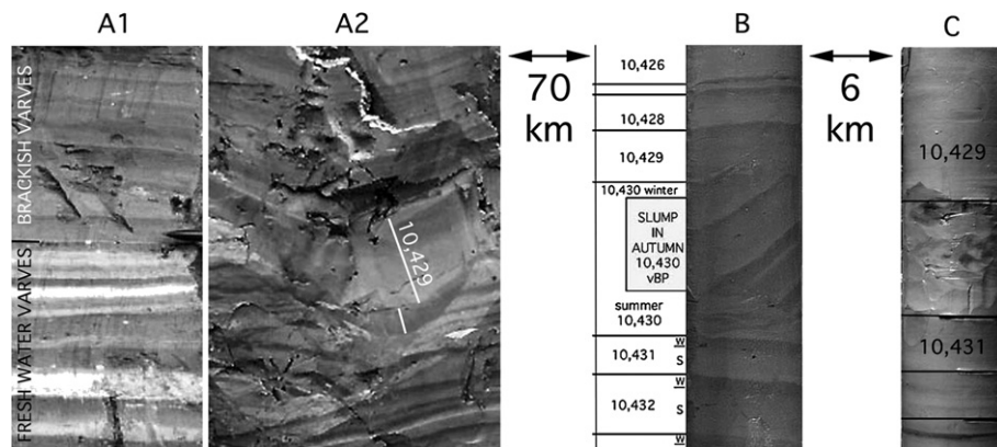
Fig. 11. Annual and seasonal recording of the 10430 vBP event at three sites; Turinge (A), Lake Albyssjön (B) and Lake Damsjön (C), spanning a distance of 76 km. A1 record the sudden switch from freshwater to brackish environment in varve 10,430. A2 records the shaking deformation and erosion with calm conditions restored in the winter of varve 10,430, indicating that the event took place in the autumn. B records a slump that entered in the autumn sequence into varve 10,430. C was first thought not to record the event, but when cleaned recorded strongly irregular (shaken) structures in the autumn part (the summer and winter units remaining homogenous).
