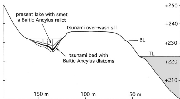
Fig. 7. The situation at Lake Källsjön (+232 m). This lake was located above the highest Baltic level (BL at +231.3 m). The sill in-between had an original level of about +236 m. At the time of the 9663 vBP tsunami, the Baltic level was at +223.5 m (TL). In the lake bed, there is a sandy tsunami bed (in fining-upward sequence) that contains a Baltic Ancyclus Lake diatom flora. In order to enter the lake basin, the tsunami wave must have been more the 12.5 m high and to have over-washed a sill at +236 m for about 700 m. Therefore, the tsunami wave is likely to have been, at least, 15 m high. In today's lake, a small fish, smelt, is living, which is likely to be a relict from the Ancyclus Lake water washed into the lake by the tsunami.
