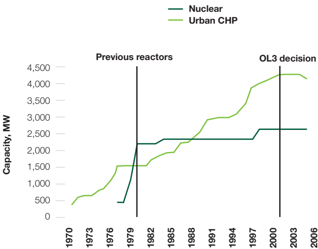
Figure 3 Impact of nuclear construction on Finnish Combined Heat and Power market
